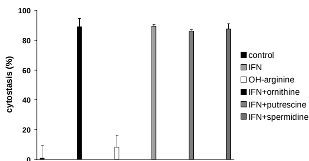
Figure 3 Cytostatic activity of IFN- \gamma , N G -hydroxy-L-arginine and the effect of polyamines on IFN- \gamma -induced cytos-tasis. NMP-1 cells were seeded at 10^4 cells/well into 96-well plates in RPMI 1640 with 10% fetal calf serum and cultured overnight. The next day, the cells were washed with phosphate buffered salines, and the medium was replaced with a low-arginine, serum-free medium (5% bovine serum albumin, 1.5% Iscove's modified Dulbecco's medium [GIBCO], 0.2% glucose, 0.01% magnesium sulfate, 0.016% calcium chloride, transferrin 5.5 \mu g/ml, and insulin 4 \mu g/ml in Hank's balanced salt medium [GIBCO], pH 7.4) alone or with rIFN- \gamma (500 U/ml). The arginine concentration of this medium was 6 \mu M, lower than plasma concentration (normal range, 50–126 \mu M [38]. After another 24 hours, rIFN- \gamma (500 U/ml), N G -hydroxy-L-arginine (250 \mu M), or rIFN- \gamma plus ornithine (1 mM), putrescine (1 mM), or spermidine (0.5 mM) was added. The cells were then pulsed with [ 3 H] thymidine and incubated for another 24 hours. The cytosstatic activity was determined as described in Materials and Methods. Similar results were observed with other EOC cell lines and when experiments were done with RPMI 1640 supplemented with 10% fetal calf serum. Data shown are representative of 3 separate experiments.
