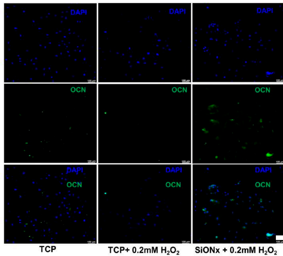
Figure 10. IHC staining representing DAPI (blue) and osteocalcin (green) on MSCs after 7 days of osteogenic differentiation. Overexpression of the osteogenic marker on the selected SiON x ( n = 1.82 ) surface vs. the control is evident. Scale bar = 100 \mu\text{m} .
